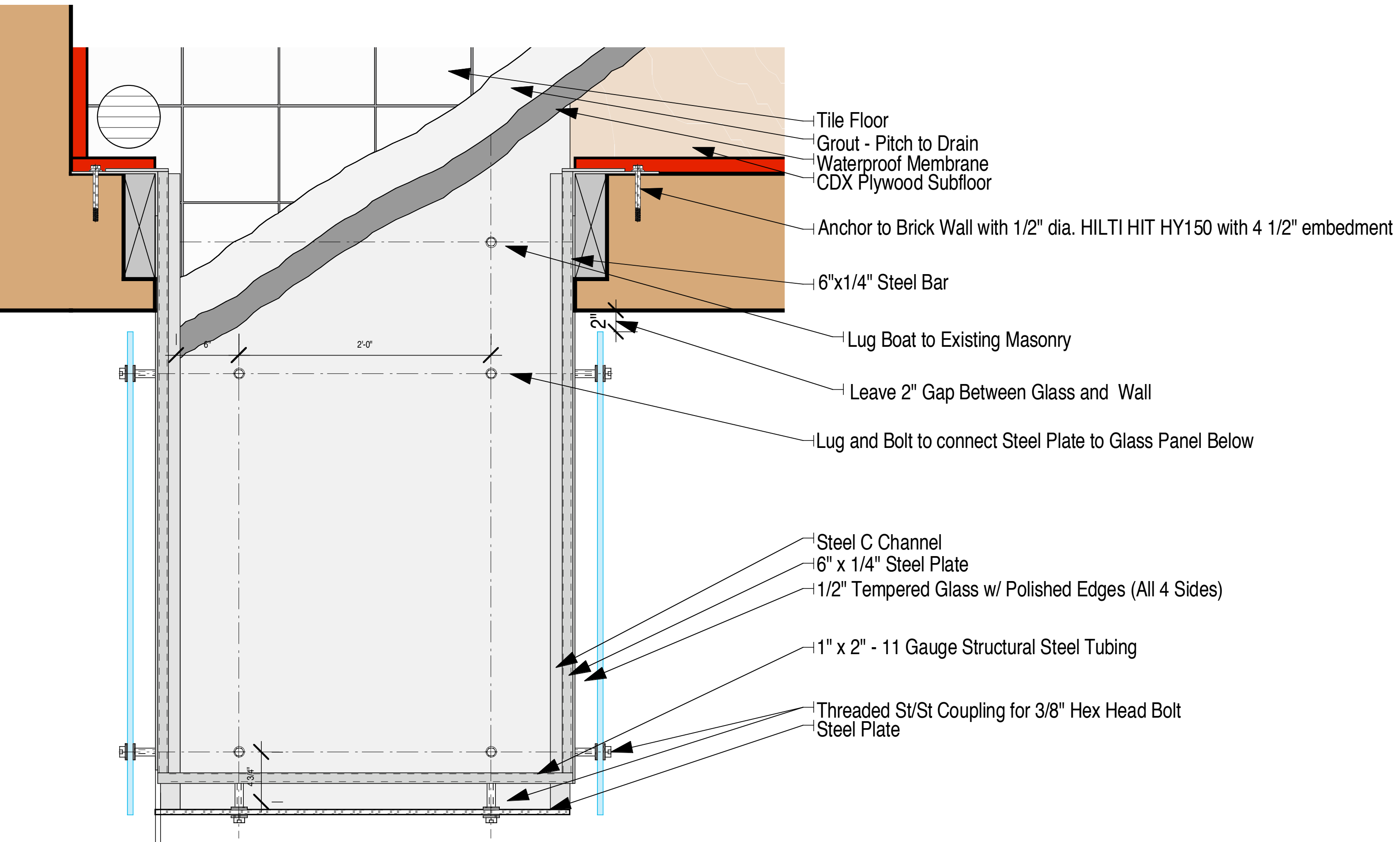
Front Glass Balconies - Plan
